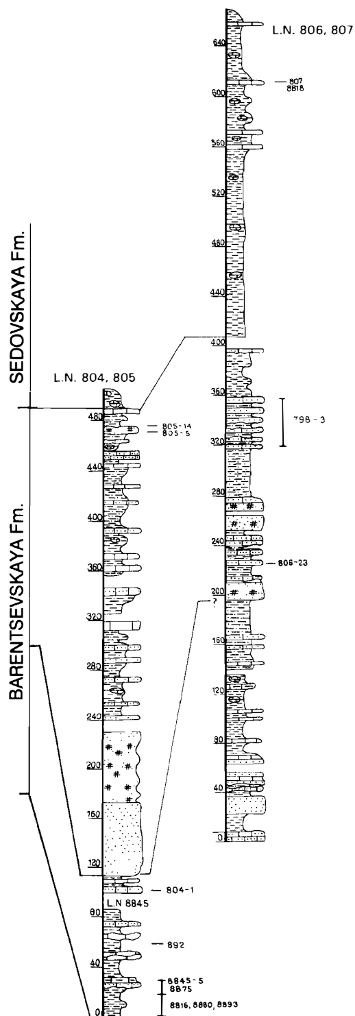
Fig. 21. Lithological sections of the Barentsevskaia and Sedovskaya formations, Litke Peninsula.
