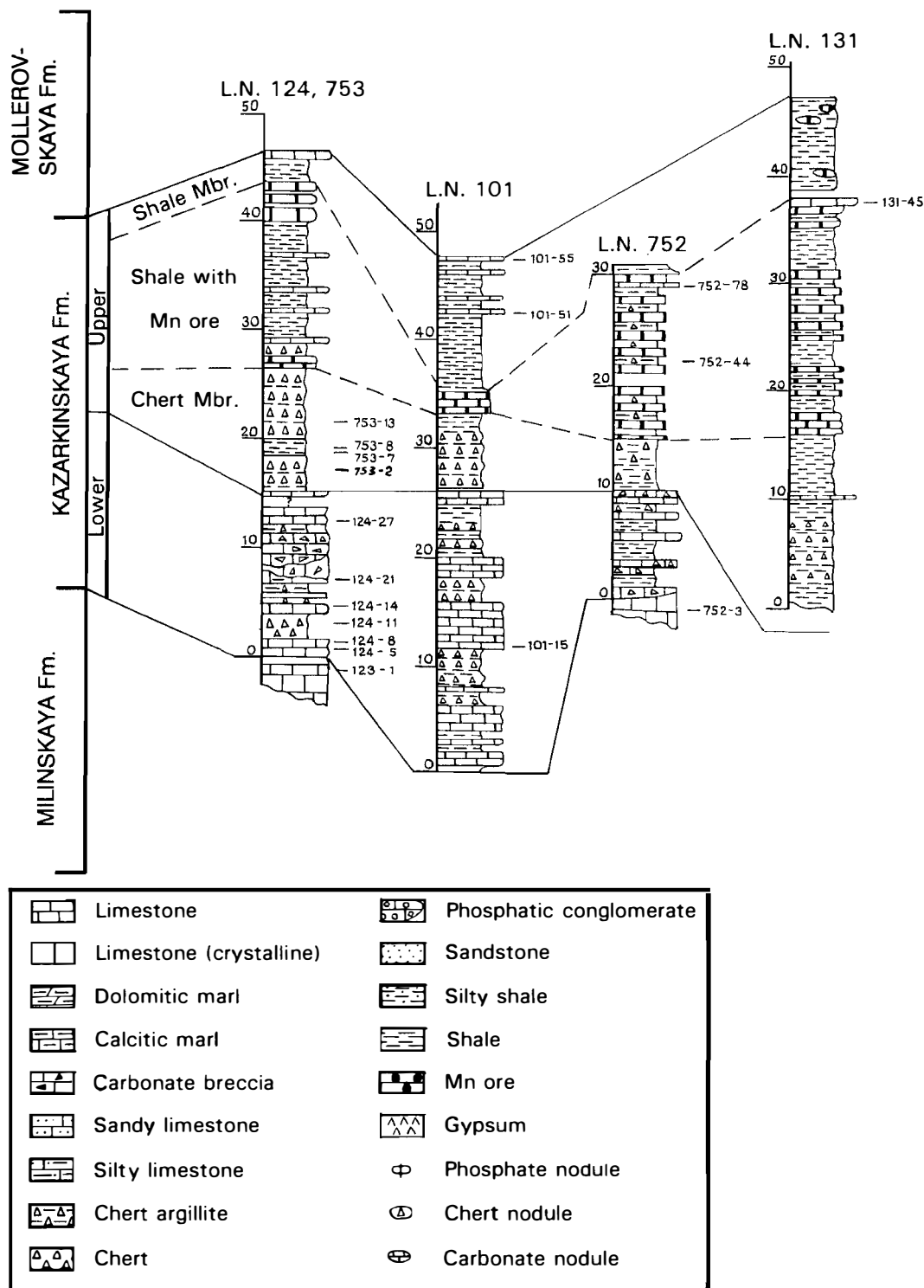
Fig. 9. Lithological sections of the Kazarkinskaya Formation. See Fig. 8 for locations.
