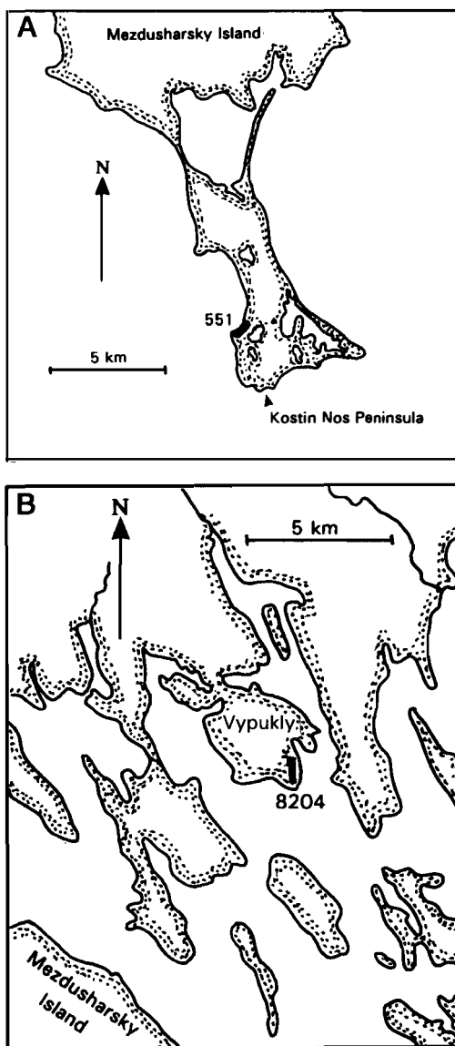
Fig. 4. Lazarevskaya Formation, Kostin-Shar Strait. A. Section 551, Mezdusharsky Island. B. Section 8204, Vypuklyi Peninsula.
