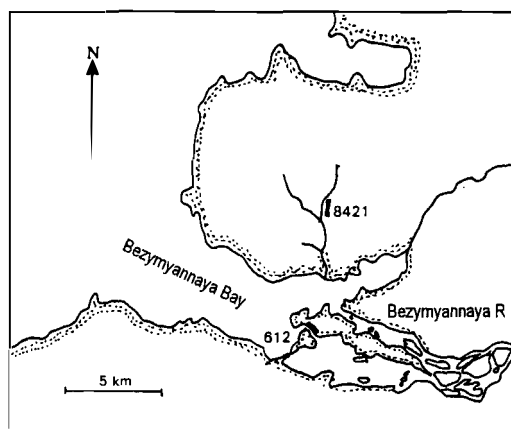
Fig. 14. Kazarkinskaya Formation, Bezymyannaya Fiord (sections 612 and 8421).
