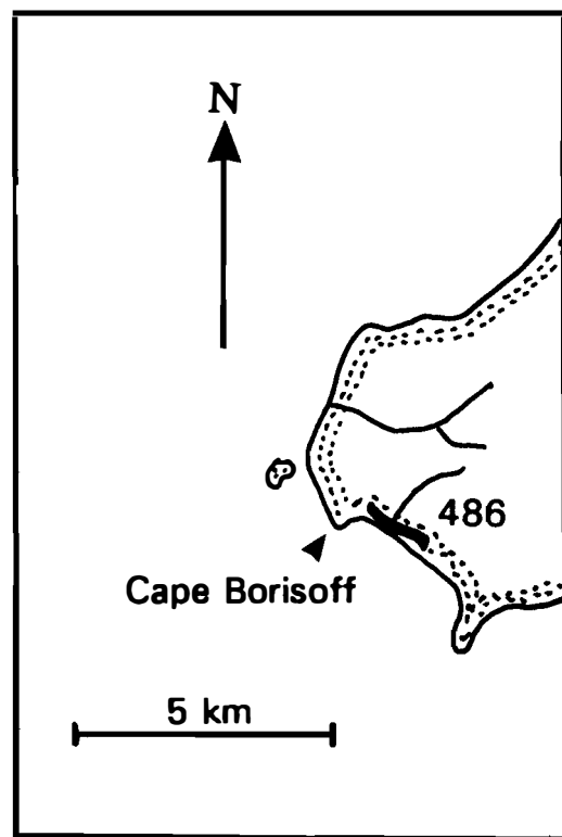
Fig. 16. Lavrovskaya Formation, Cape Borisoff (section 486).
