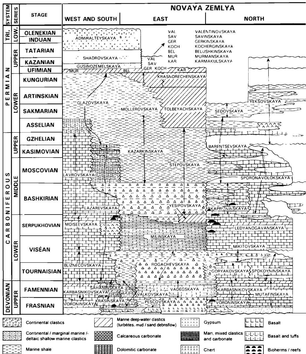
Fig. 2. Middle–Upper Palaeozoic sequences of Novaya Zemlya.
