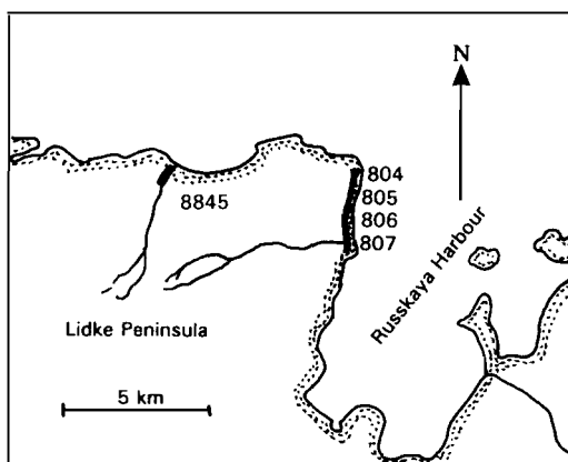
Fig. 20. Barentsevskaya and Sedovskaya formations, Litke Peninsula.
