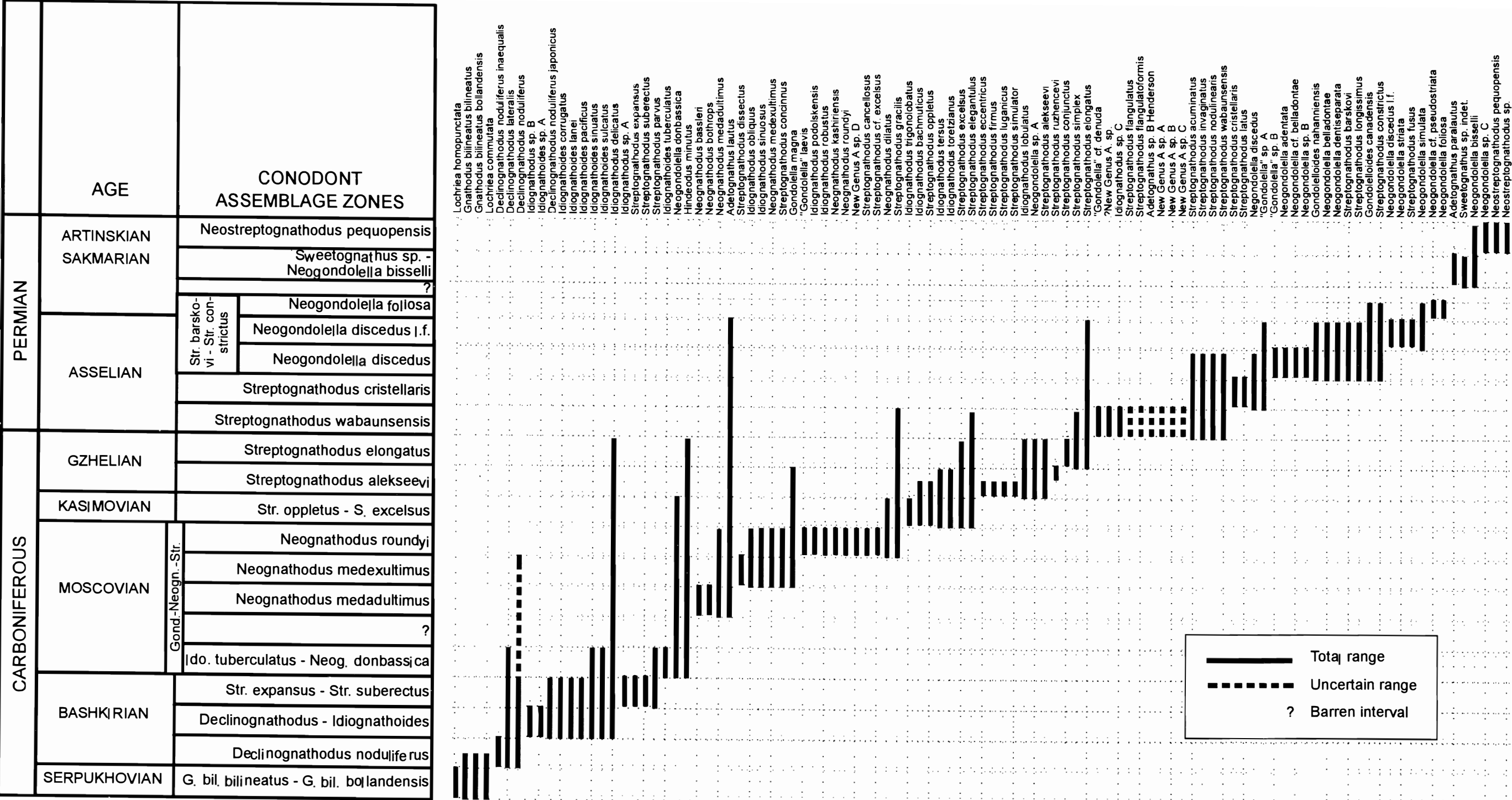
Fig. 30. Range chart showing conodont assemblage zones and stratigraphically arranged conodont distribution in composite sections in Novaya Zemlya.
