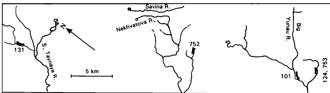
Fig. 8. Kazarkinskaya Formation localities. Bolshaya Yunau River (section 124, 753, and 101), Nekhvatoва River (section 752), and Tainaya River (section 131).
