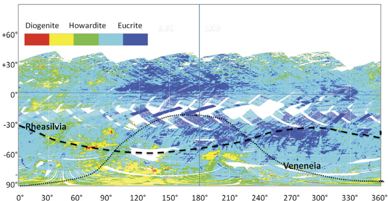
FIGURE 5 Global map of the distribution of terrains dominated by eucrite, diogenite, and howardite on Vesta, based on VIR spectra from De Sanctis et al. (2012a). The dashed and
