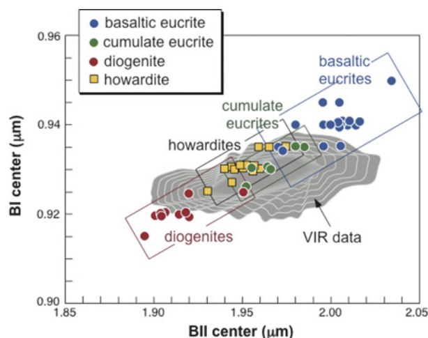
FIGURE 3 BI versus BII band center positions for spectra of HED meteorites, and a cloud of Vesta data measured by visible-light-infrared (VIR) spectroscopy. The boxes are defined by well-characterized HEDs, each having at least 30 spectral measurements.
