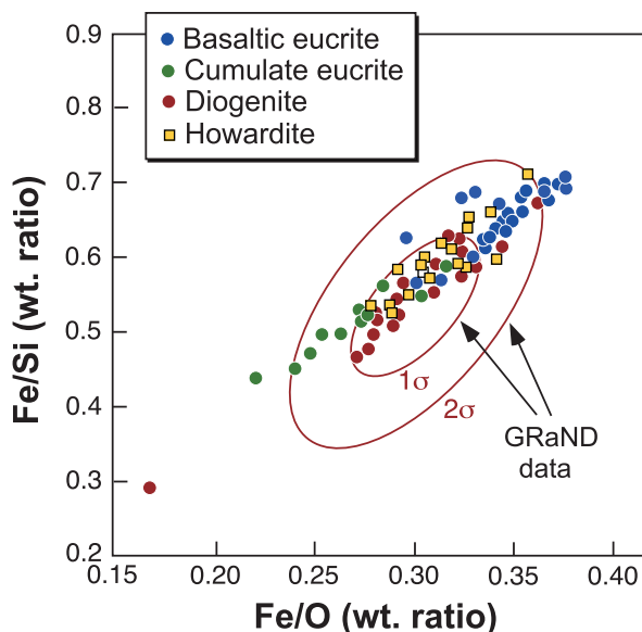
FIGURE 4 GRaND element ratios for Vesta compared to the compositions of HED meteorites. The 1\sigma and 2\sigma ovals indicate standard deviations of the mean for GRaND's Vesta data. DATA FROM PRETTYMAN ET AL. (2012)
