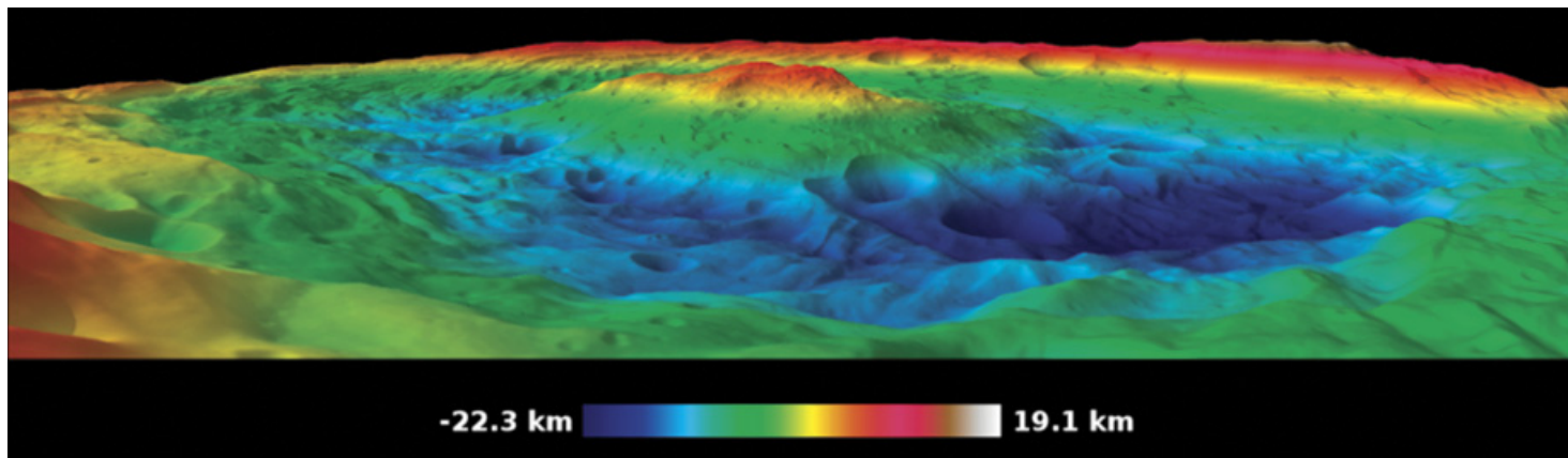
FIGURE 1 Perspective view of the topography of Vesta's south pole region, showing the huge Rheasilvia impact basin. Elevations, relative to the average Vesta surface, are indicated by coloration and demonstrate that this basin significantly affects the asteroid's overall shape. This view was compiled by the Dawn Science Team from Framing Camera images.
