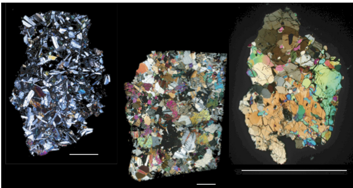
FIGURE 2 Photomicrographs (crossed polars) of ( left ) basaltic eucrite, composed of ferroan pyroxenes and plagioclase; ( center ) cumulate eucrite, composed of magnesian
