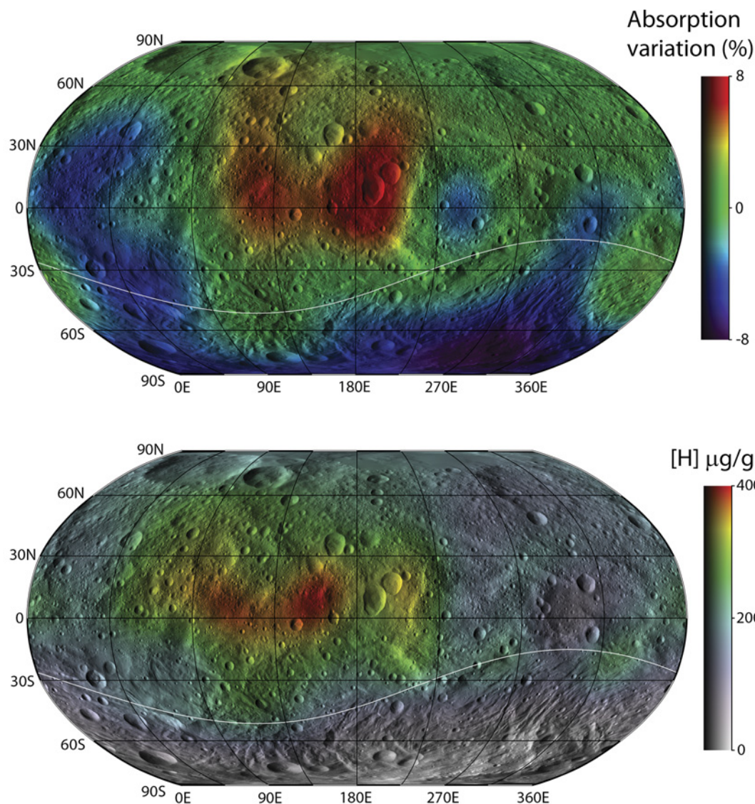
FIGURE 6 Global map of the relative variations of thermal neutron absorption measured by GRaND, confirming the identification and distribution of lithologies based on VIR spectra. Regions with low (blue) or high (red) absorption contain more diogenite or basaltic eucrite, respectively. The Rheasilvia boundary is shown by the white line. GRaND data are superimposed on a shaded relief map provided by R. Gaskell.
