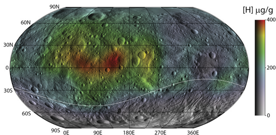
FIGURE 7 GRaND global map of hydrogen, from Prettyman et al. (2012), and a photomicrograph (crossed polars) of a howardite sample containing dark clasts of carbonaceous chondrite.
